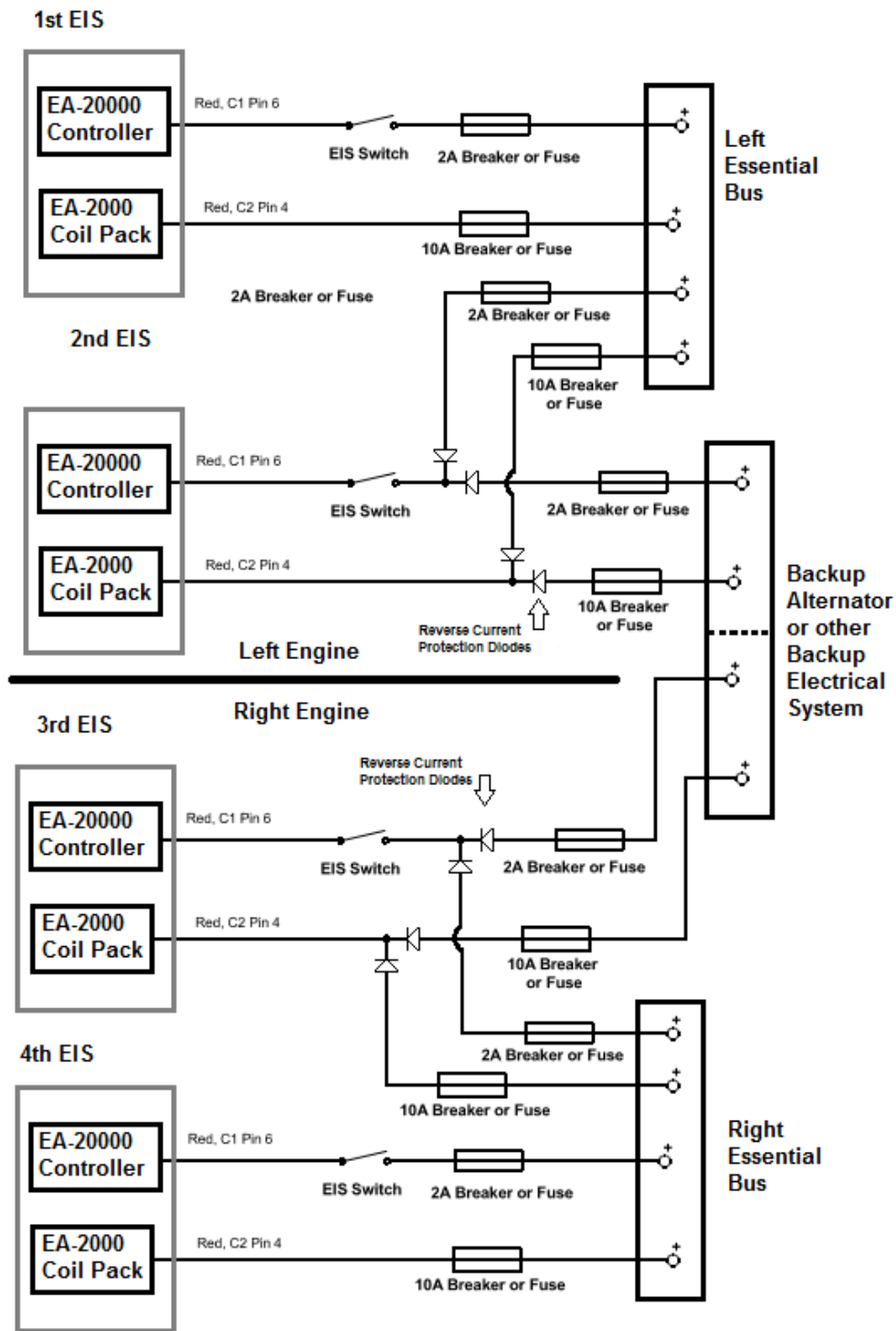
Figure 8: Twin Engine, Dual EIS, Single Electrical System Power Connections
