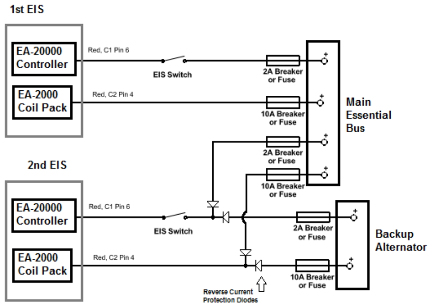
Figure 6: Single Engine, Dual EIS Backup Alternator Connections
